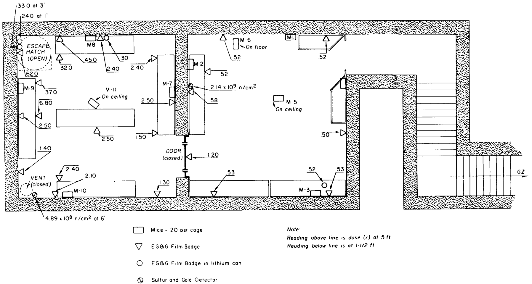
Fig. 5—Locations and types of measurements recorded by various radiation dosimeters inside shelter 8001.
